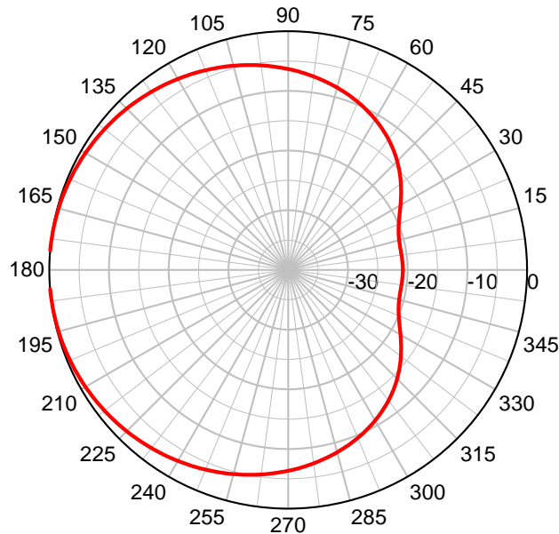
ODR-2400T120K – Azimuth Plot
