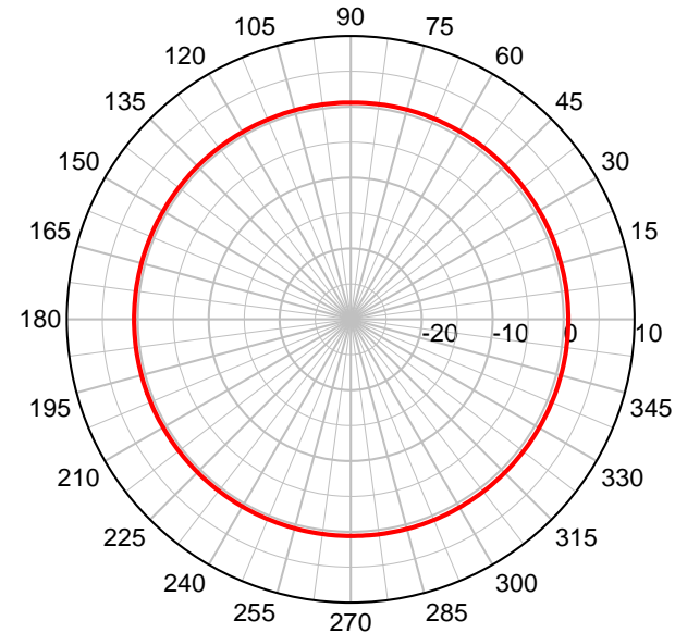
MG0 @ 1900 MHz – Azimuth Plot
